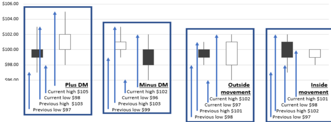
Plus and Minus Directional Movement Indicators
